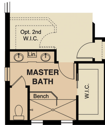
OPTIONAL MASTER BATH LAYOUT 3
